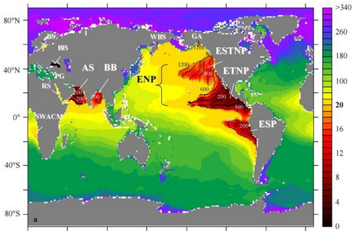
Figure 1-5. Map of O_2 distribution at depth where O_2 concentration is minimal ( O_2 in \mu M ) throughout Earth's oceans, taken from Fig. 1 of (Paulmier and Ruiz-Pino 2009). Oxygen minimum zones are pointed out in white letters: Arabian Sea (AS), Bay of Bengal (BB), Black Sea (BIS), Baltic Sea (BS), Eastern Northern Pacific (ENP), Eastern South Pacific (ESP), Eastern Sub-Tropical North Pacific (ESTNP), Eastern Tropical North Pacific (ETNP), Gulf of Alaska (GA), Persian Gulf (PG), Red Sea (RS), South Western African Continental Margin (SWACM), and Western Bering Sea (WBS).
