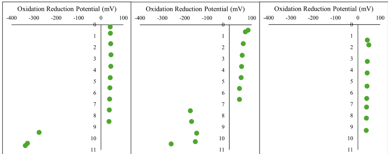
Figure 3. Oxidation reduction potential from the Salton Sea water column in August 2020 (left), September 2021 (middle), and November 2023 (right). Y-axis represents water column depth in all graphs.
