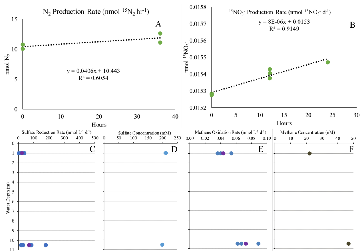
Figure 4-4. Microbial respiration rates from the November 2023 sampling campaign. (A) N_2 production rate at 10.5 m depth in the lake, used to calculate denitrification rates. (B) NO_3^- production rate at 10.5 m depth in the lake, used to calculate annamox rates. (C) Sulfate reduction rates at 1 m and 10.5 m depth (same as Fig.4-2I). (D) Sulfate concentrations at 1 m and 10.5 m depth (same as 2J). (E) Methane oxidation rates at 1 m and 10.5 m depth. Blue dots represent discrete samples while purple dots represent average per depth. (F) Methane concentrations at 1 m and 10.5 m depth.
