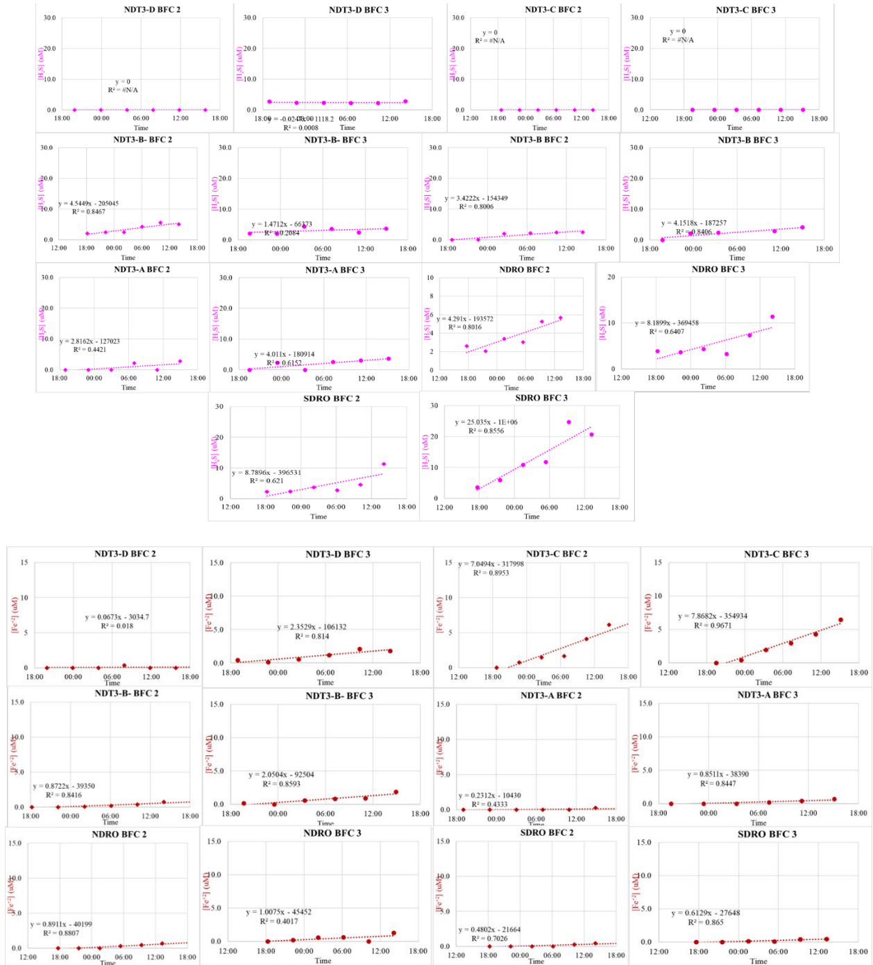
Figure 5. Changes in sulfide (top) and Fe^{2+} (bottom) over time used to construct benthic fluxes from individual chambers in 2023.
