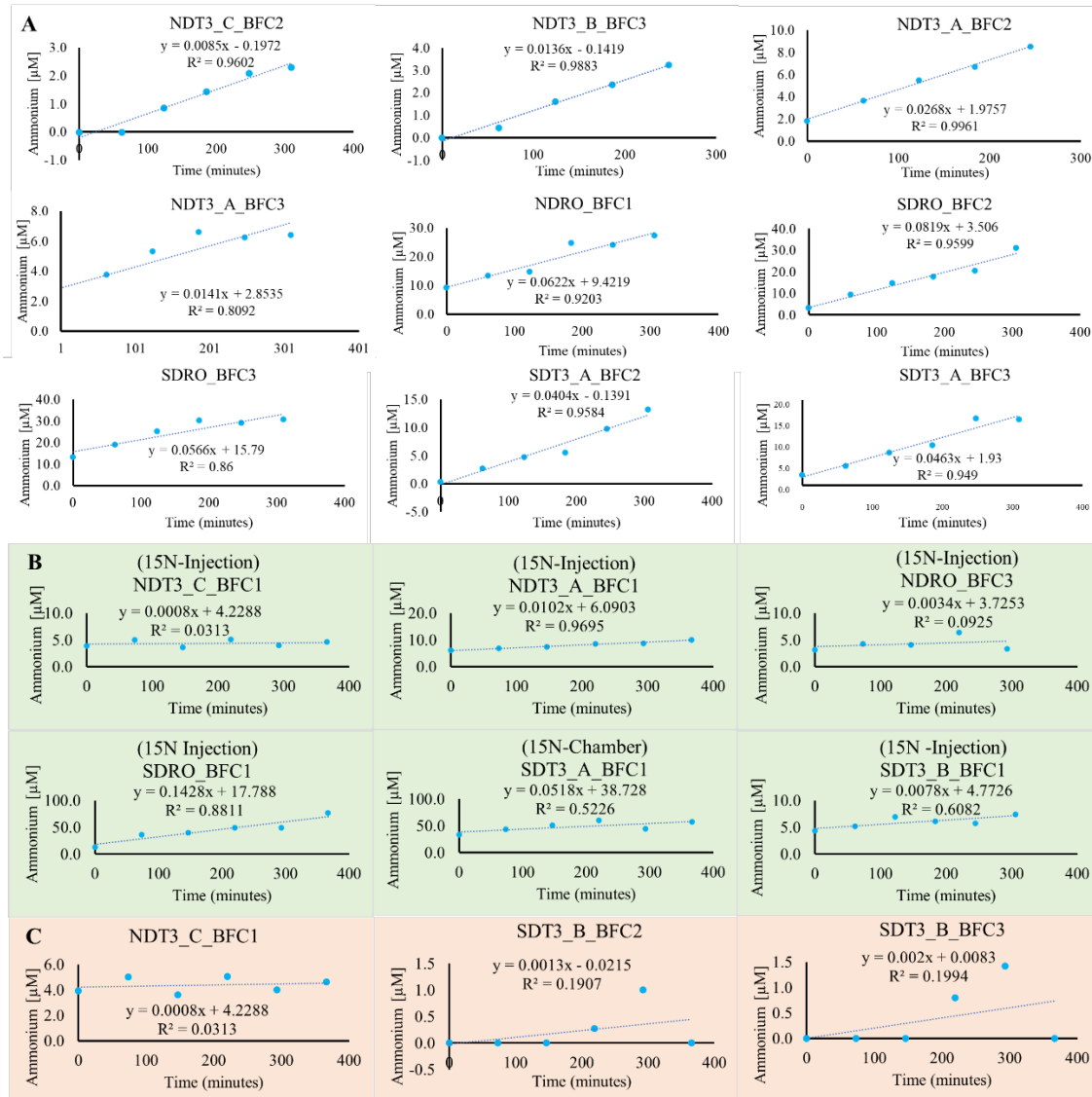
Figure 1: A) Ammonium concentration changes over time from benthic flux chamber (BFC1, BFC2, BFC3) incubations. B) Ammonium concentration changes over time from ^{15}\text{N} -Nitrate benthic flux chamber incubations. Note these chambers were not used to calculate benthic fluxes. C) Ammonium concentration changes over time from benthic flux chamber incubations where there was no calculatable flux. No data are shown from chambers if there was a mechanical failure with the deployment or ammonium concentrations were all below detection. For station abbreviation definitions please refer to the main manuscript.
