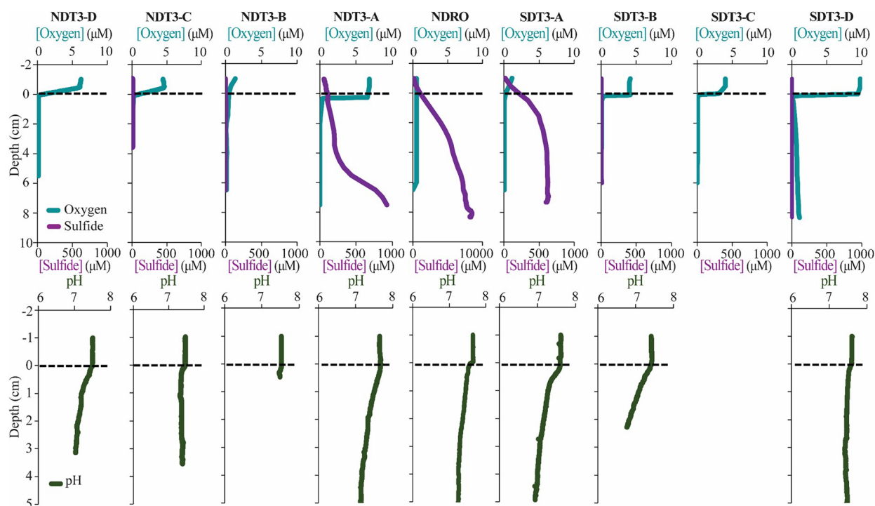
Figure 2-4. In-situ sediment microprofiler results for all stations (except SDT1-A and SDRO): oxygen ( O_2 ) and total sulfide (sulfide) concentration in the first row; pH profiles in the second row. Note the change in scale on the secondary x-axis for NDRO sulfide. Values determined in the overlying water are plotted at negative sediment depths; the dotted line connotes the sediment-water interface.
