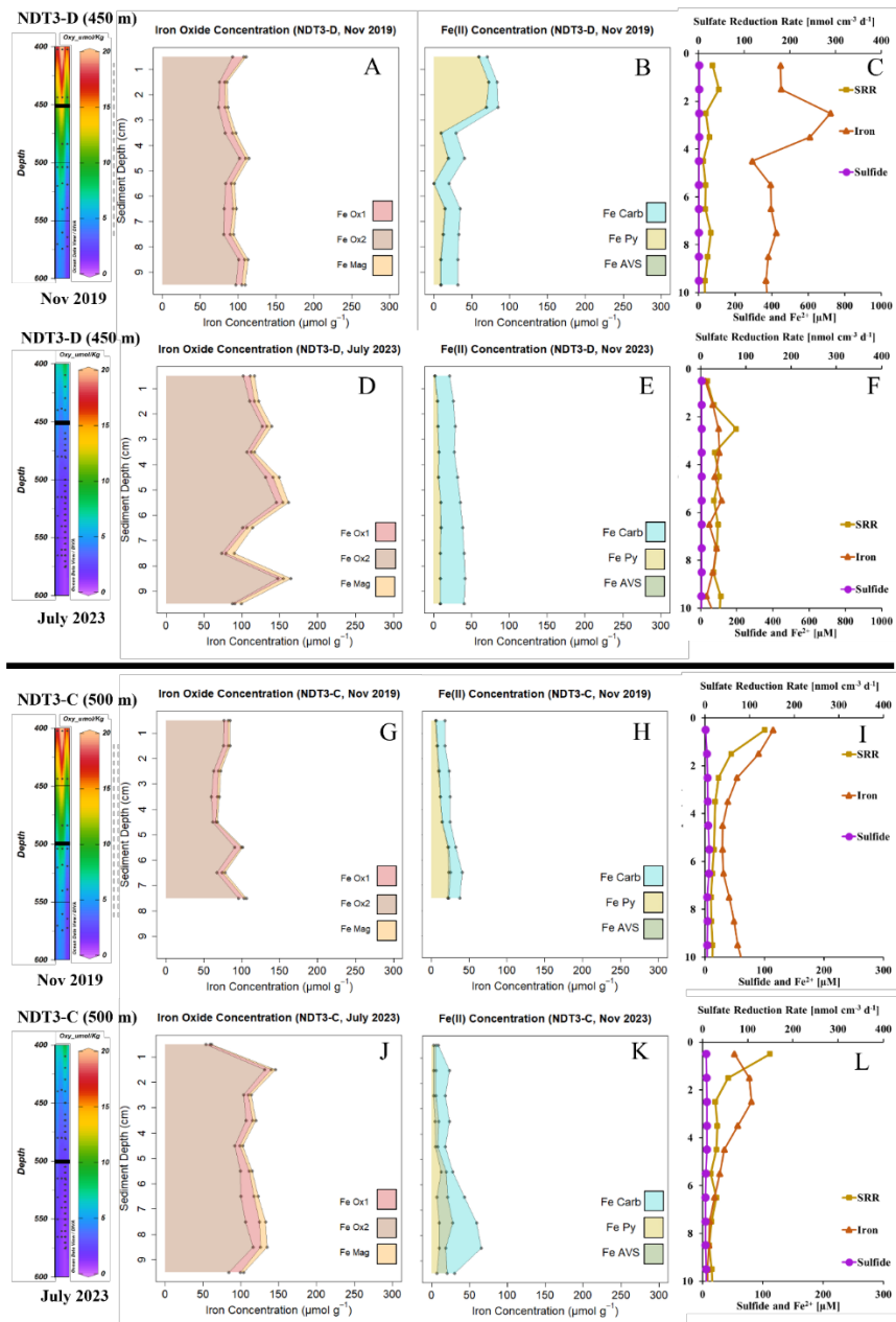
Figure 3-3: Sediment iron minerals and parameters relevant for their formation.
