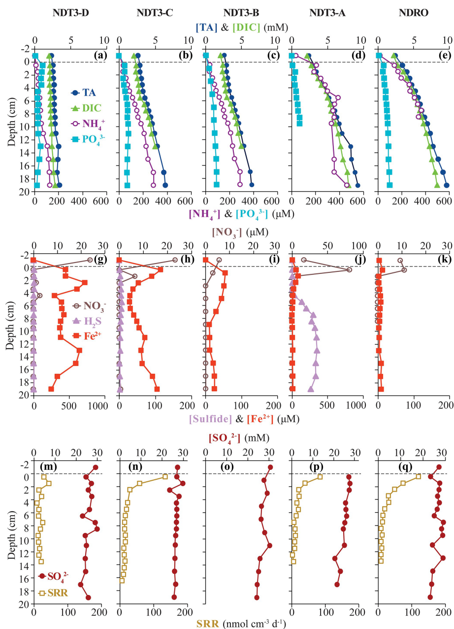
Figure 2-2. Biogeochemical data from ROV sediment push cores collected at stations on the northern transect (NDT3) and in the northern depocenter (NDRO): total alkalinity (TA), dissolved inorganic carbon (DIC), ammonium ( \text{NH}_4^+ ), phosphate ( \text{PO}_4^{3-} ) in the first row; nitrate ( \text{NO}_3^- ), total sulfide (sulfide), and iron (II) ( \text{Fe}^{2+} ) in the second row; sulfate ( \text{SO}_4^{2-} ) and bacterial sulfate reduction rate (SRR) in the third row. Data analyzed from sediment core supernatant are plotted at -1 cm sediment depth; the dotted line connotes the sediment-water interface. Note the change in scale on the primary x-axis in panel I and the change in scale of the secondary x-axis in panels F and I. No spectrophotometric sulfide data is available for NDRO and NDT3-B and no SRR data is available for NDT3-B. For station details see Fig. 1 and Table 1.
