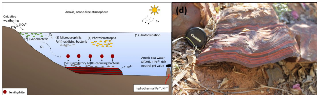
Figure 1-1. Left: Schematic of the genesis of banded iron formation. 1) Photooxidation of Fe^{2+} provides Fe^{3+} in Precambrian Oceans. 2) Weathering of continental crust provides nutrients for cyanobacteria growth in the photic zone, producing O_2 as a byproduct. 3) Some of the O_2 from these cyanobacteria provides the oxidant for iron-oxidizing bacteria, generating Fe^{3+} . 4) Oxidation of Fe^{2+} to Fe^{3+} by photoferrotrophs performing anoxygenic photosynthesis. 5) Some O_2 from step (2) combines with Fe^{3+} to form iron oxides (e.g., ferrihydrite), an insoluble solid which settles on the seafloor. Some of these iron oxides are reduced to mixed valence iron (e.g., magnetite) or back to Fe^{2+} , some of which could be re-oxidized by processes (1), (3), or (4). Right: A representative banded iron formation from Western Australia. Taken from Figs. 1 & 2 from Dreher et al. (2021).
