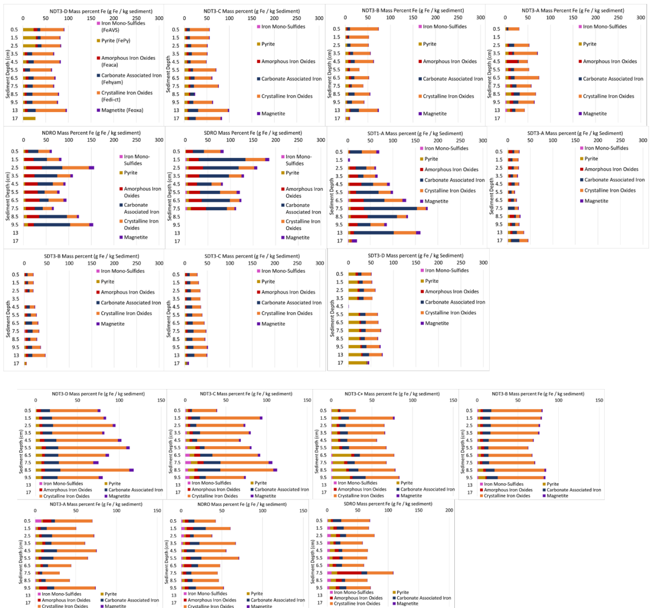
Figure 4. Sediment digestions from 2019 (top cluster) and 2023 (bottom cluster). Each bar represents a discrete depth. Iron concentrations are shown as g Fe per kg of sediment.
