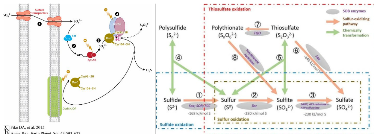
Figure 1-4. Left: Schematic of sulfate reduction, taken from (Fike et al. 2015). 1) Sulfate is transported into the cell using a sulfate transporter (or via passive diffusion). 2) Sulfate is reduced to APS. 3) APS is reduced to sulfite. 4) The DSR protein complex reduces sulfite to thiosulfate and hydrogen sulfide. DsrC then acts as an electron acceptor in the electron transport chain of sulfate-reducing bacteria. Right: Schematic of common microbial sulfur oxidation pathways, taken from (Cui et al. 2019). Focusing on the transformation of sulfide to sulfate: 1) Oxidation of sulfide to elemental sulfur via Sox, SQR, or FCC enzymes. 2) Oxidation of elemental sulfur to sulfite by Dsr enzyme. 3) Oxidation of sulfite to sulfate by APS reductase and ATP sulfurylase.
