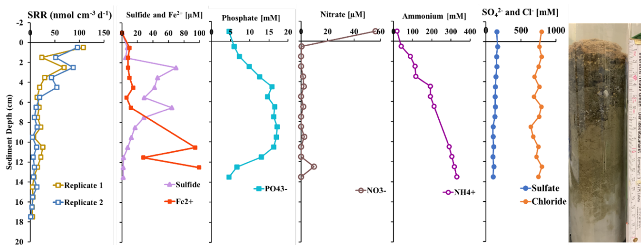
Figure 4-3. Biogeochemical parameters in Salton Sea sediment from the sampling campaign to the south basin depocenter in August 2021. Starting from left to right: sulfate reduction rate (SRR); sulfide and iron concentrations; phosphate concentrations; nitrate concentrations; ammonium concentrations; sulfate and chloride concentrations; and a photo of the core used for sulfate reduction rates. The two SRR replicates represent different sub-cores from the same core.
