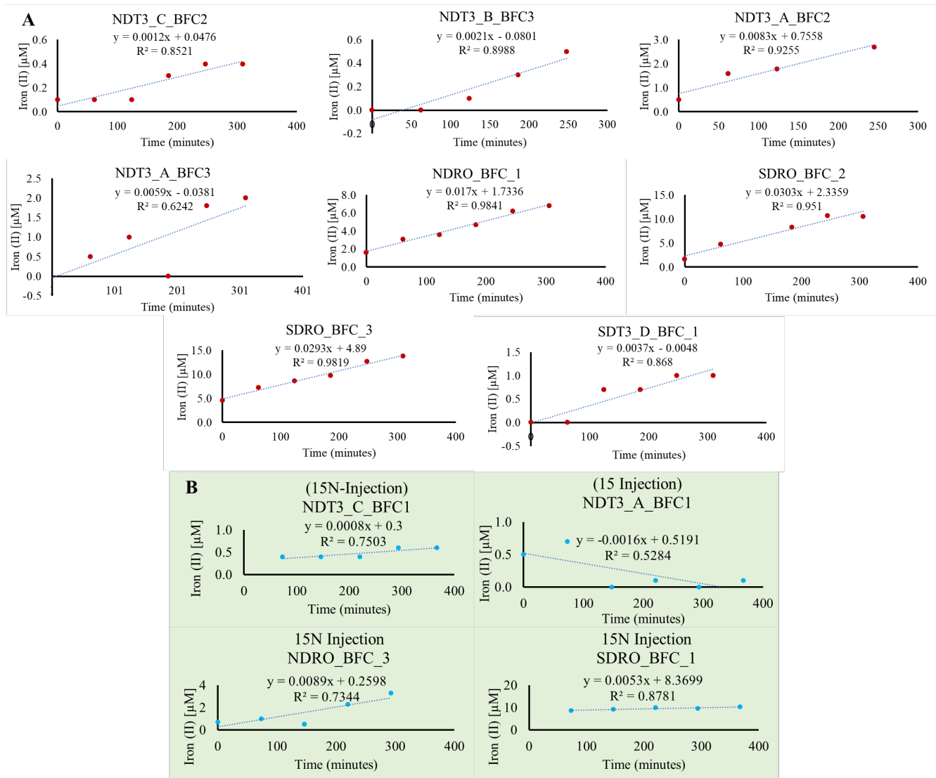
Figure 3: Iron (II) concentration changes over time from benthic flux chamber (BFC1, BFC2, BFC3) incubations. B) Iron (II) concentration changes over time from ^{15}\text{N} -Nitrate benthic flux chamber incubations. Note these chambers were not used to calculate benthic fluxes. No data are shown from chambers if there was a mechanical failure with the deployment or concentrations were all below detection. For station abbreviation definitions please refer to the main manuscript.
